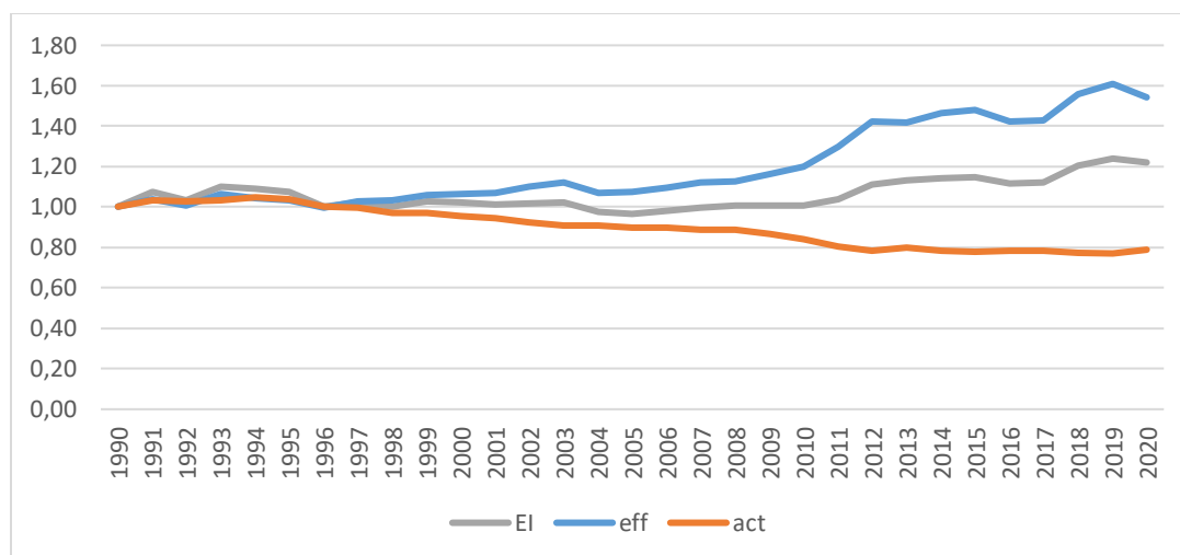
Figure 2 Decomposition of EI in Algeria (1990 base year)
