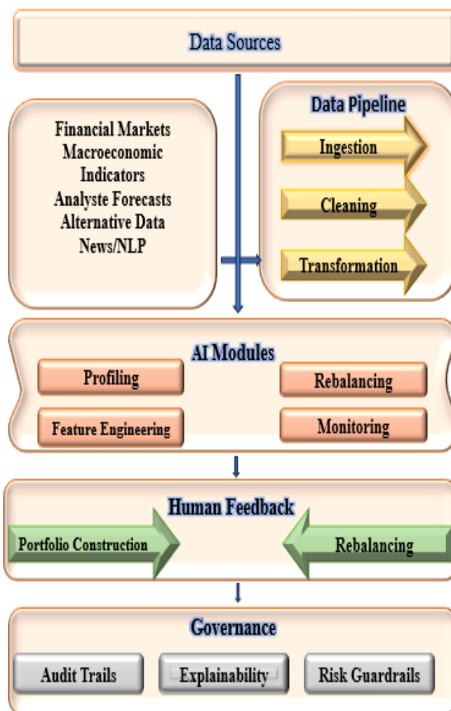
Figure 1 Robo-advisor architecture
