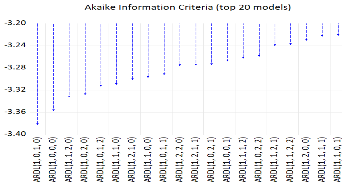
Figure 1 Optimal lag length selection results
