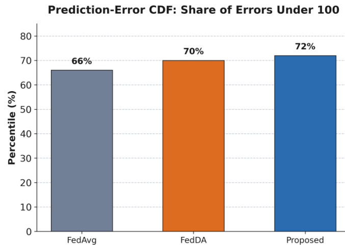
Figure 6 Prediction-error
