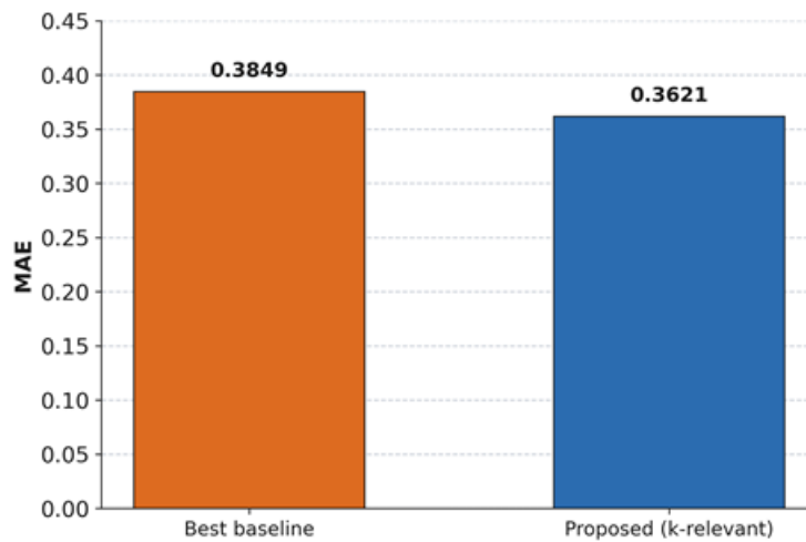
Figure 3 MAE prediction with dataset 2
