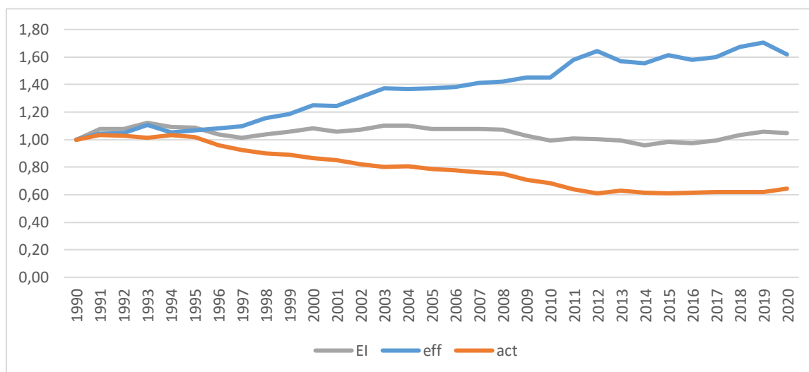
Figure 3 Decomposition of the final EI in Algeria (1990 base year)
