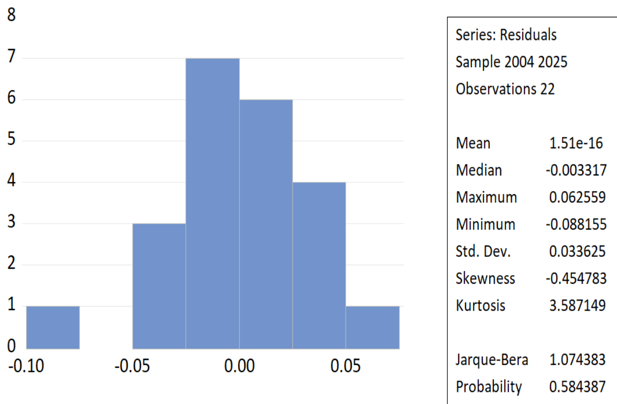
Figure 2 Normality test - histogram jarque-bera
