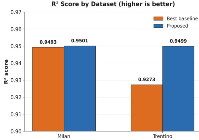
Figure 4 R 2 score based on given dataset
